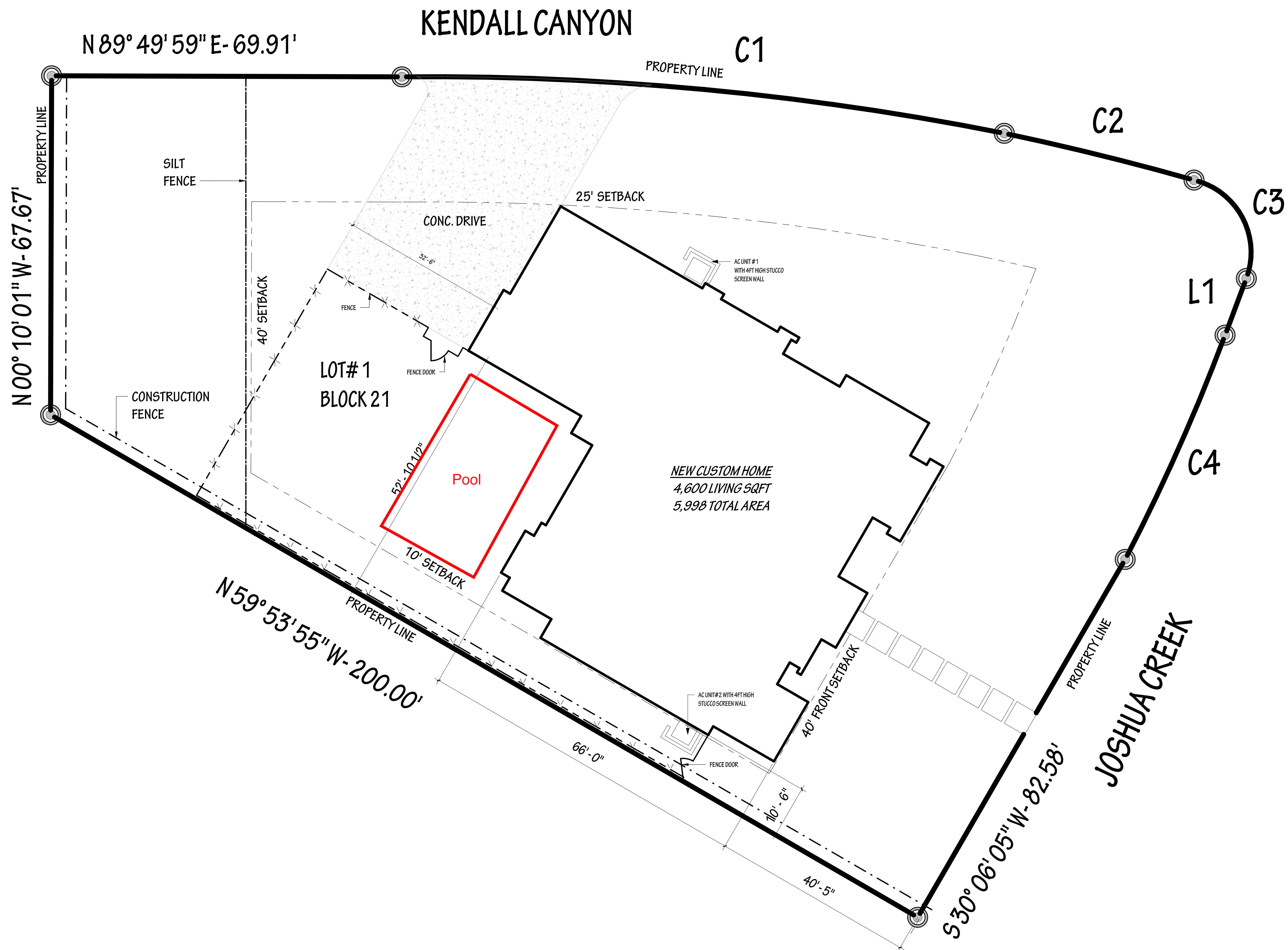
1 SITE PLAN AS1.1 1" = 10'-0"
